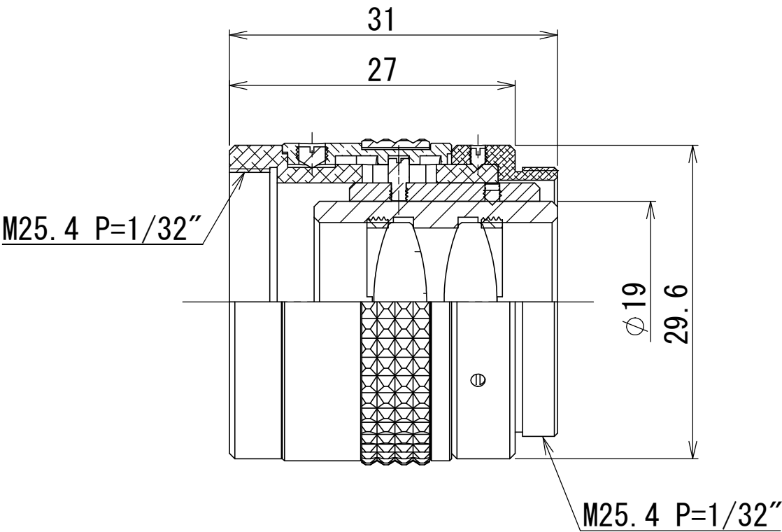
※レンズ鏡筒を組み込んだ場合の構造図 * Structural drawing with the lens barrel incorporated
